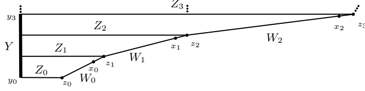
FIGURE 3. (\rho_1, 2) -contraction
