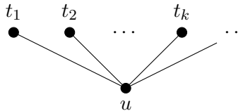
FIGURE 2. A fan (t_k)_{k \in \omega} and its corresponding \wedge -root u .
