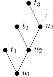
FIGURE 1. A comb (t_k)_{k \in \omega} and its corresponding \wedge -chain (u_k)_k .
